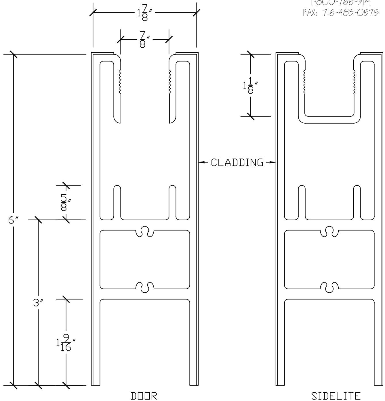
6" SQUARE RAIL FOR 3/4" GLASS
