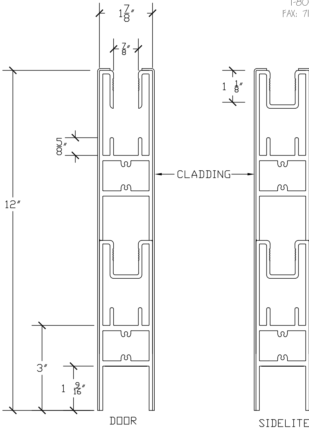
12" SQUARE RAIL FOR 3/4" GLASS (HALF SCALE)
