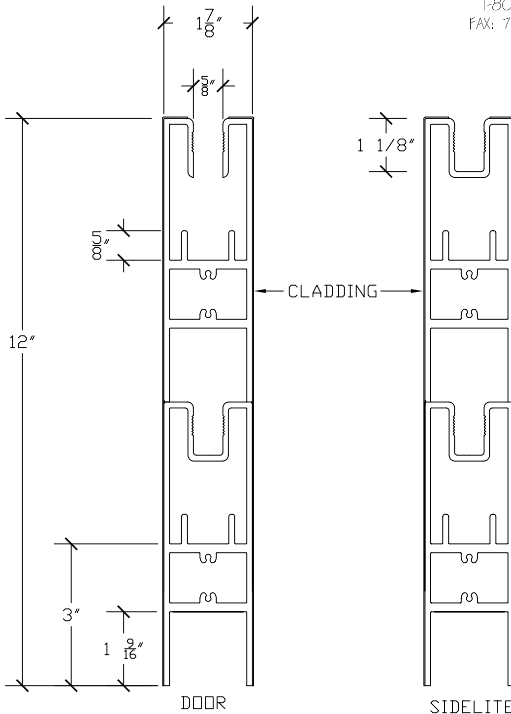
12" SQUARE RAIL FOR 1/2" GLASS (HALF SCALE)
