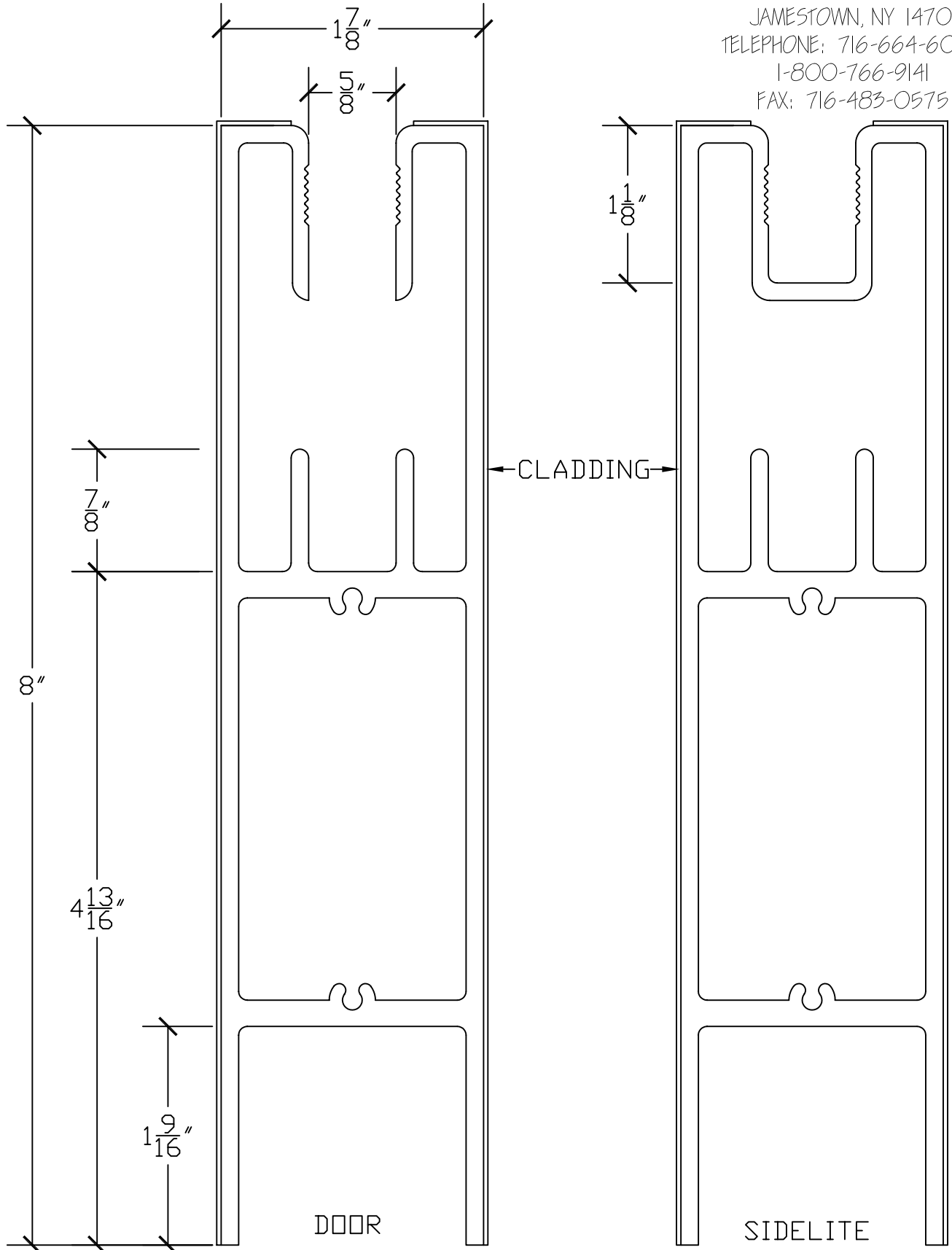
8' SQUARE RAIL FOR 1/2" GLASS
