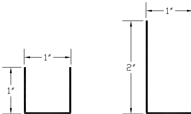
BRASS AND STAINLESS STEEL U-CHANNELS
