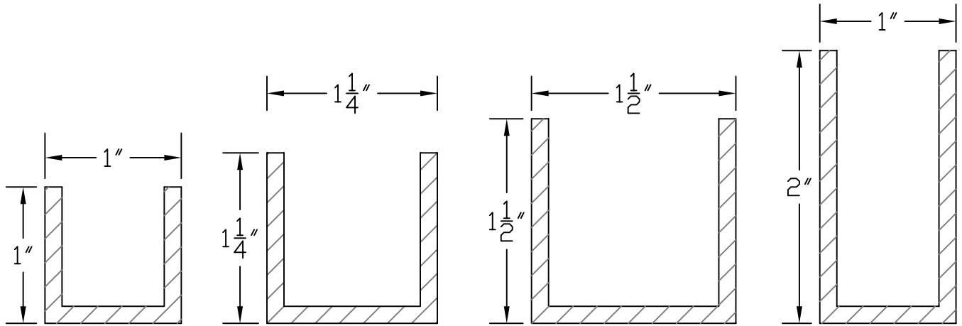
ALUMINUM CHANNELS
